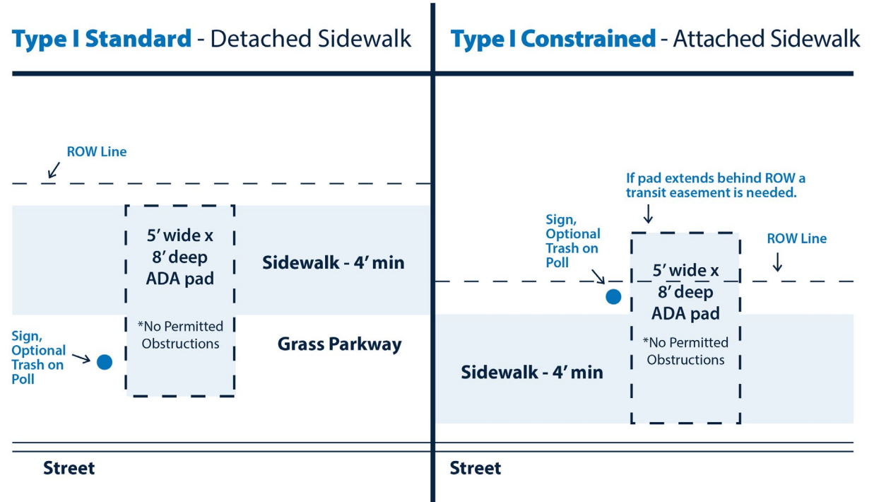
Figure 13: Type 1 Standard and Type 1 Constrained Stop
