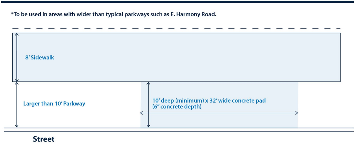
Figure 21: Type III Wide Parkway (Detached Sidewalk)
