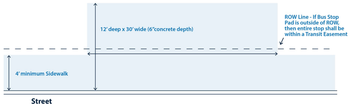
Figure 19: Type III Constrained (Attached Sidewalk)
