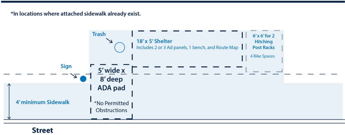
Figure 20: Type III Constrained (Attached Sidewalk) – Amenity Detail
